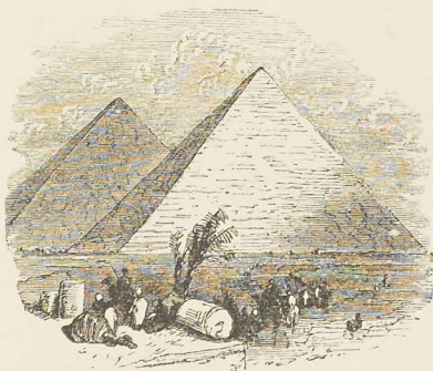
LIMESTONE PYRAMIDS.
